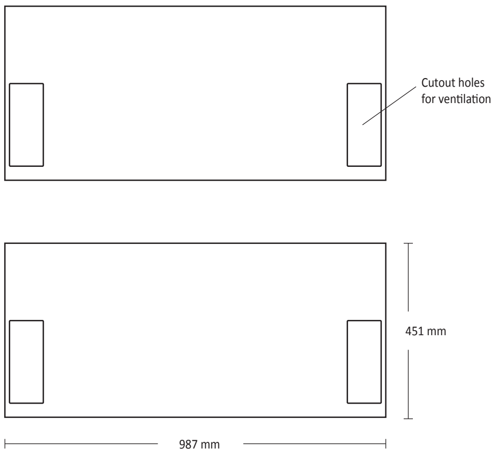
Left and right sides Scale 1:10
